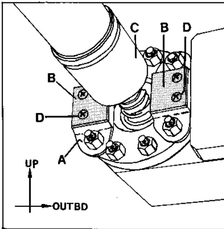
Figure 1 Mechanical Down Stop
